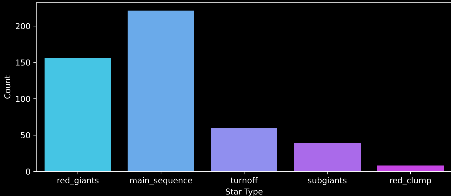
APOGEE DR17 Field: [320+45] Count plot of Star Type
