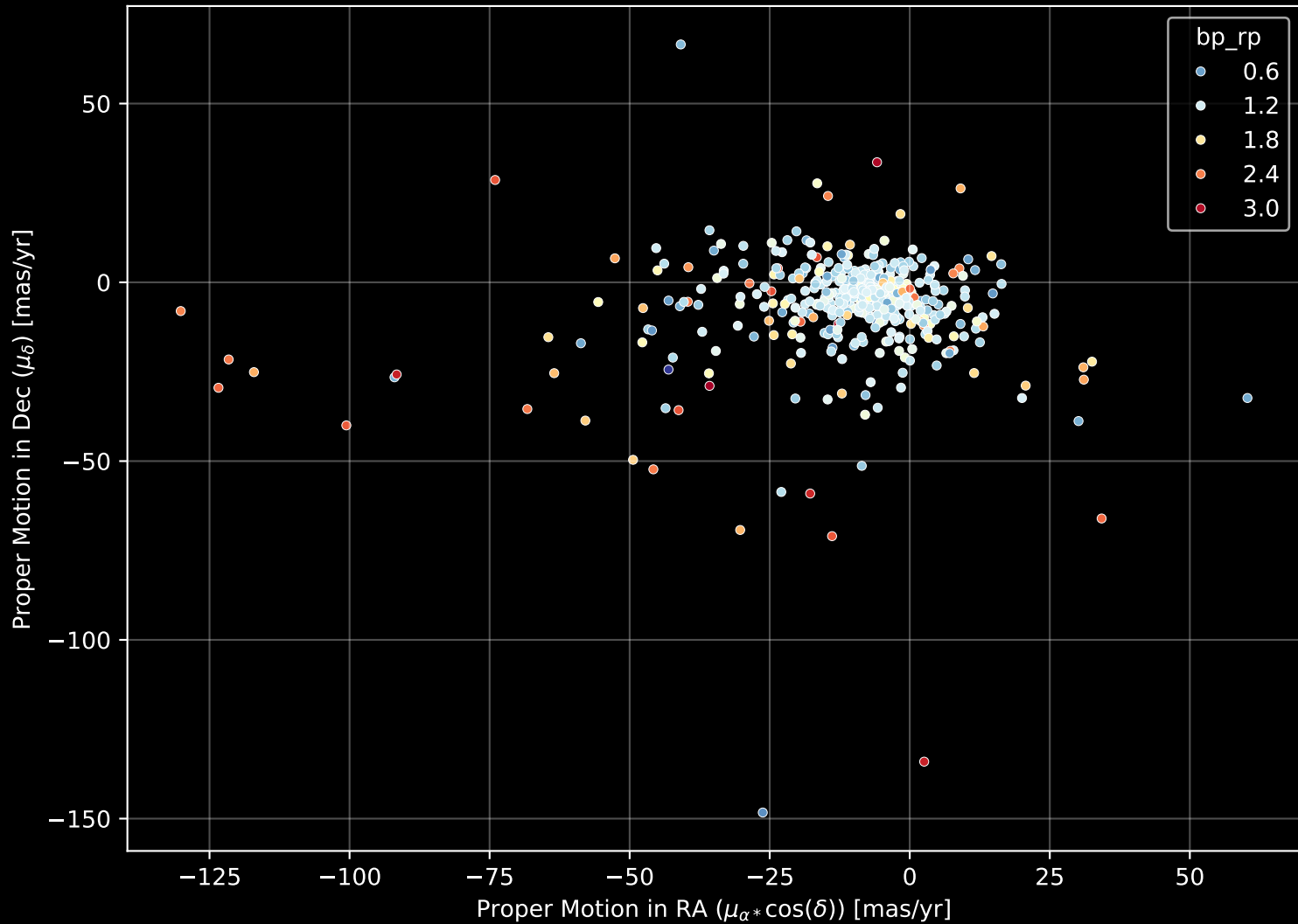
APOGEE DR17 Field: [320+45] Proper Motion Diagram (n= 483)
