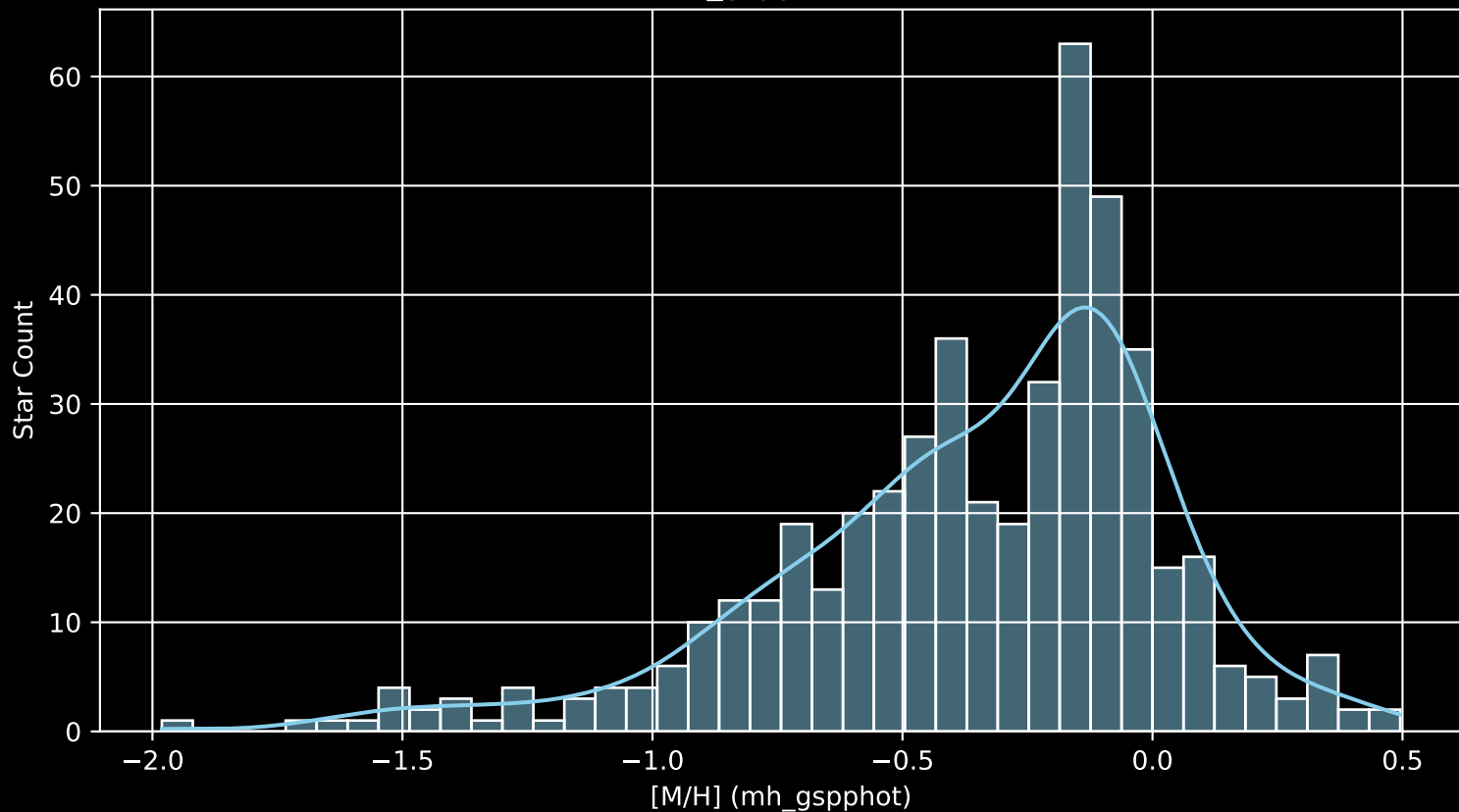
APOGEE DR17 Field: [320+45 [M/H] (mh_gspphot) (n= 482)
