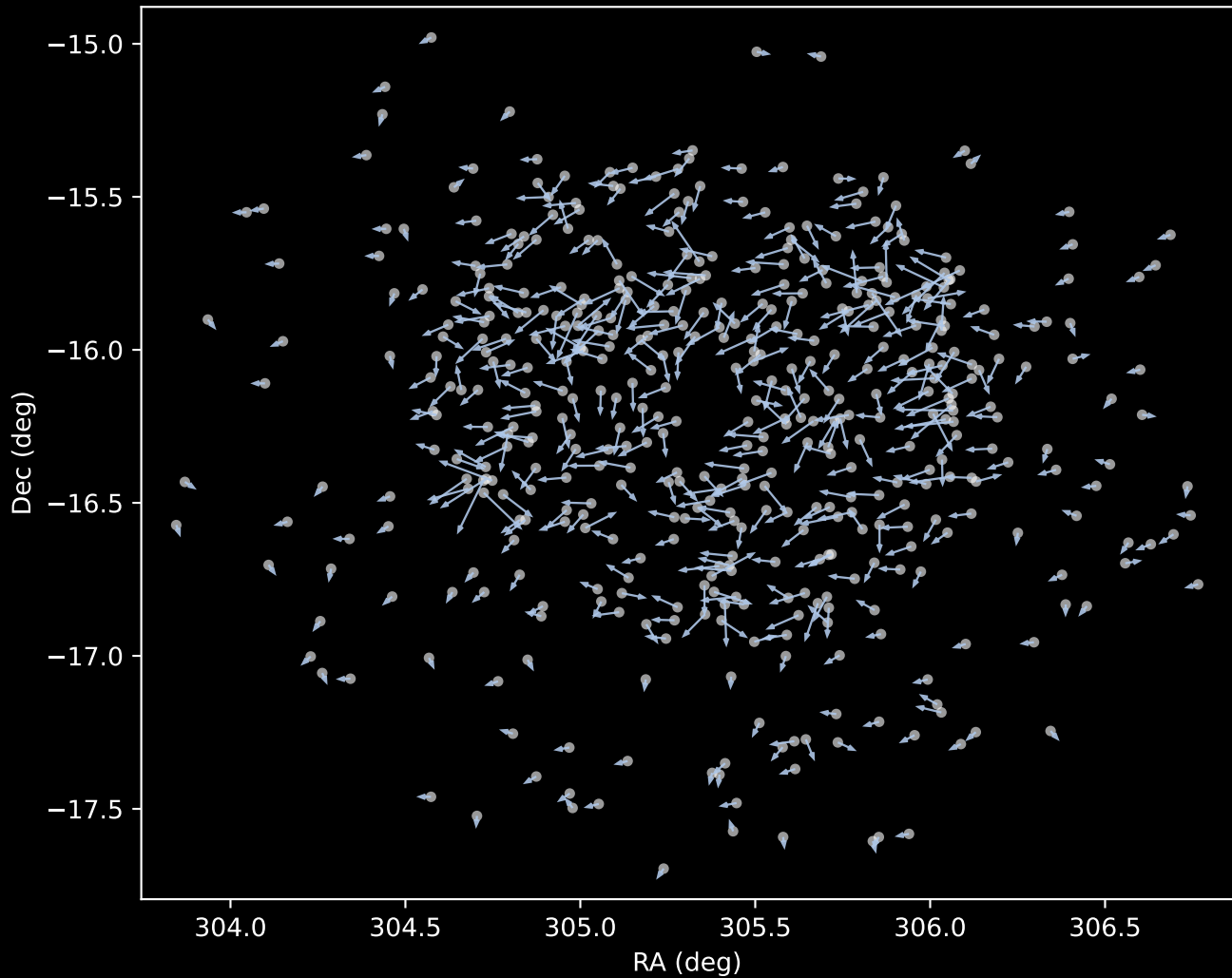
APOGEE DR17 Cluster 1 Proper Motion Vectors (n=470)
