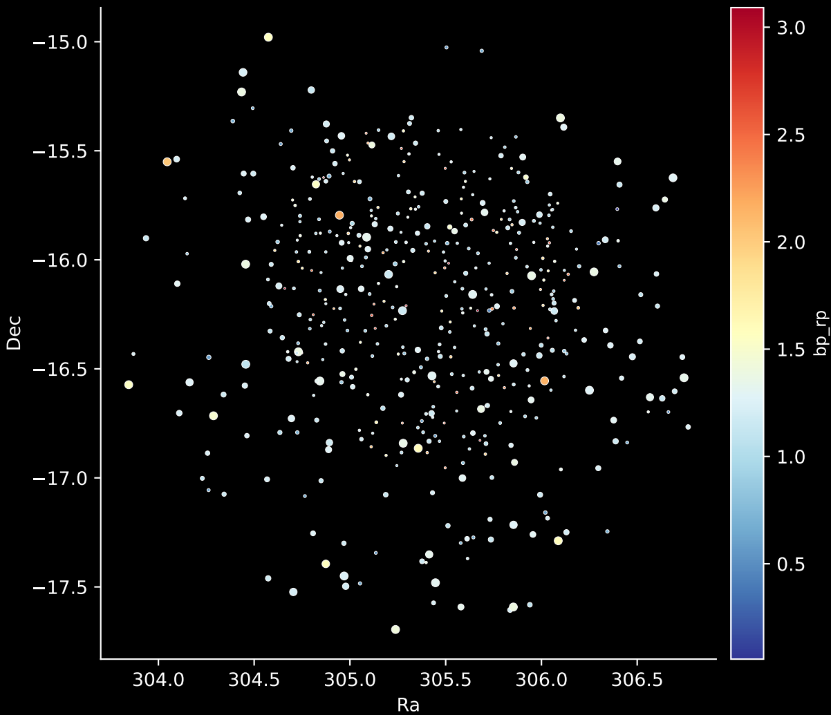
APOGEE DR17 Field: [320+45] Stars: 483
