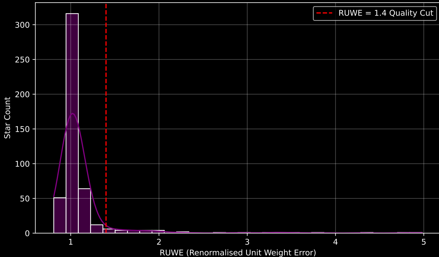
GAPOGEE DR17 Field [320+45] RUWE Distribution (n= 476)
