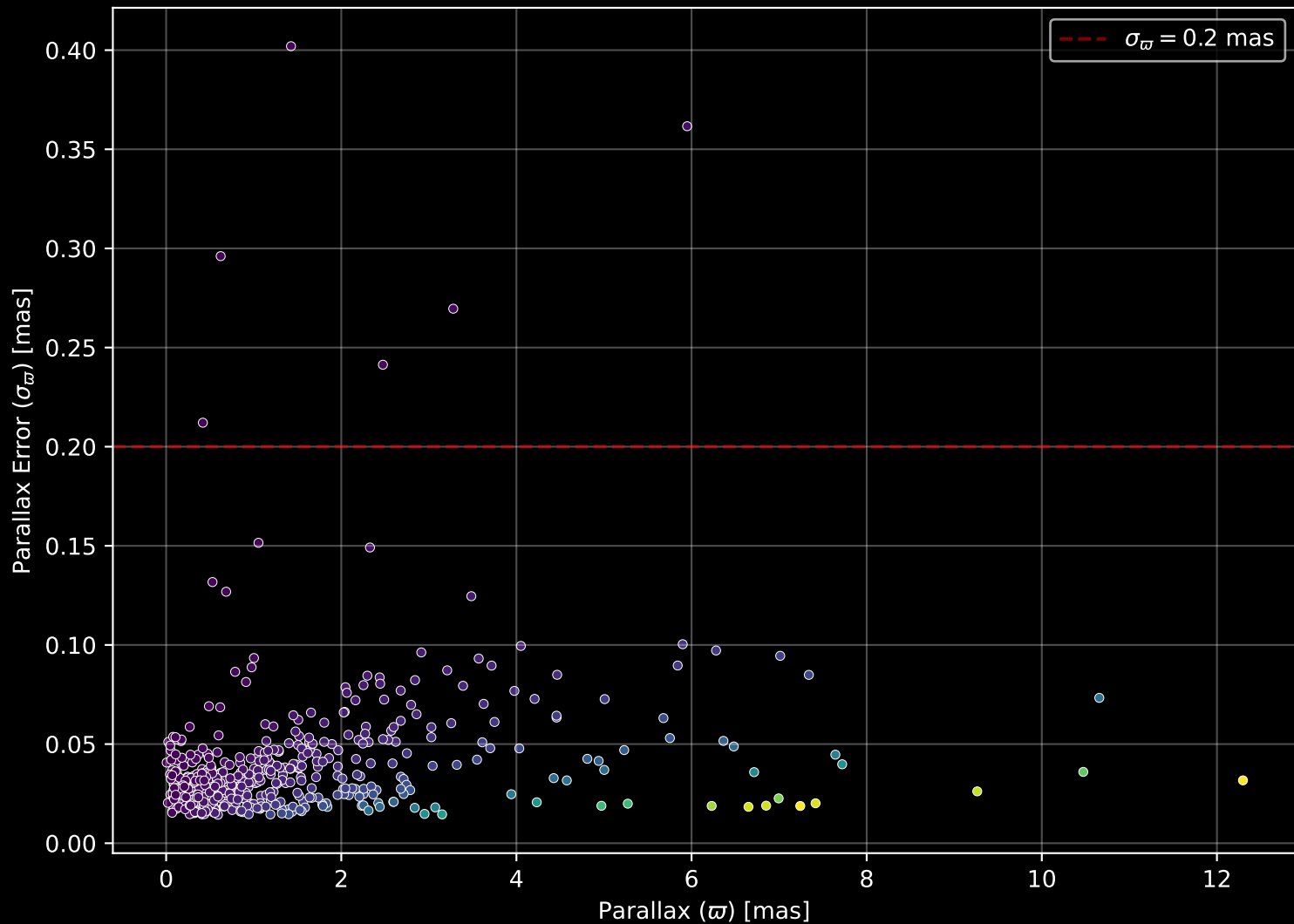
APOGEE DR17 Field: [320+45] Parallax Quality (n= 483)
